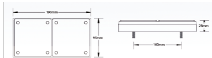
Part No 280ARM Stop/Tail/Indicator
